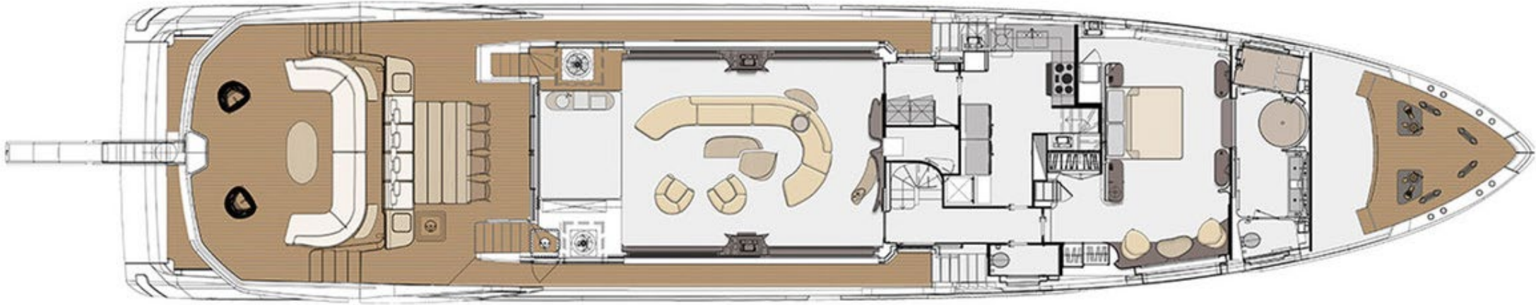
MAIN DECK
