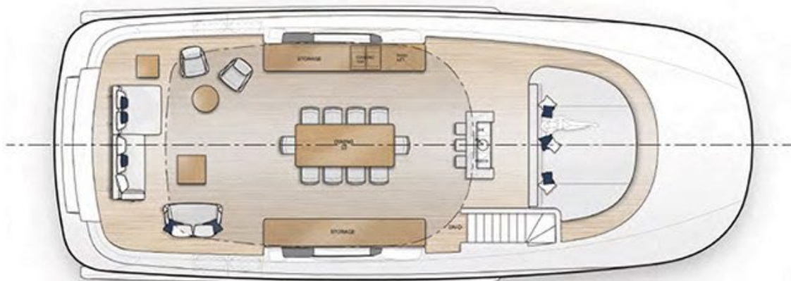
OASIS 40M Sun deck | Proposed configuration
