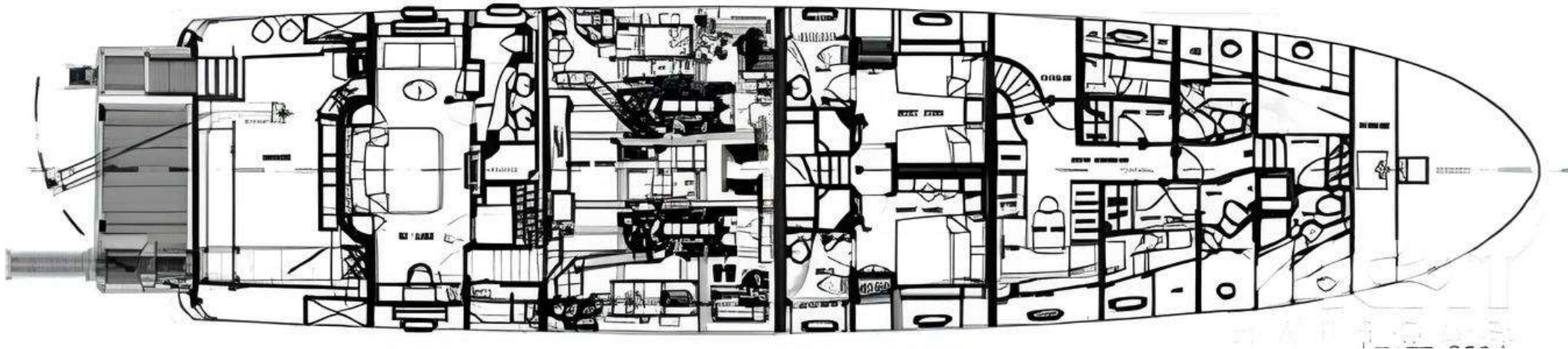
UPPER DECK
