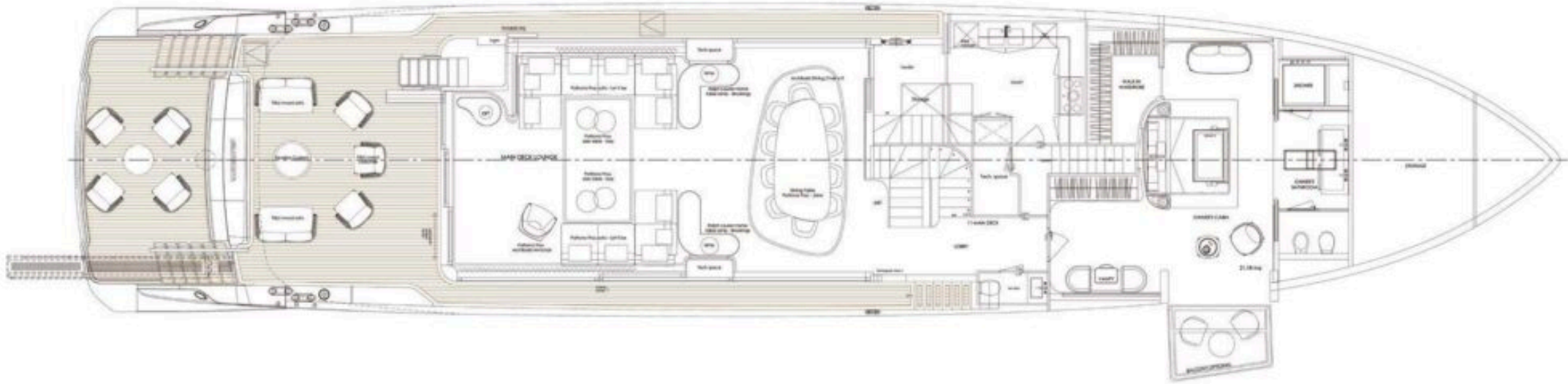
MAIN DECK
