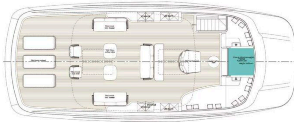
SUNDECK
