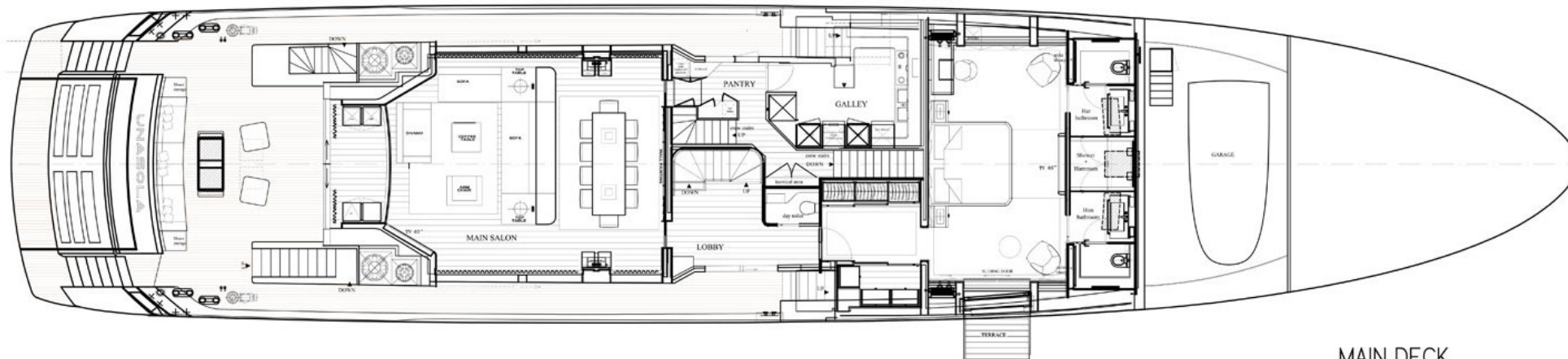
MAIN DECK
