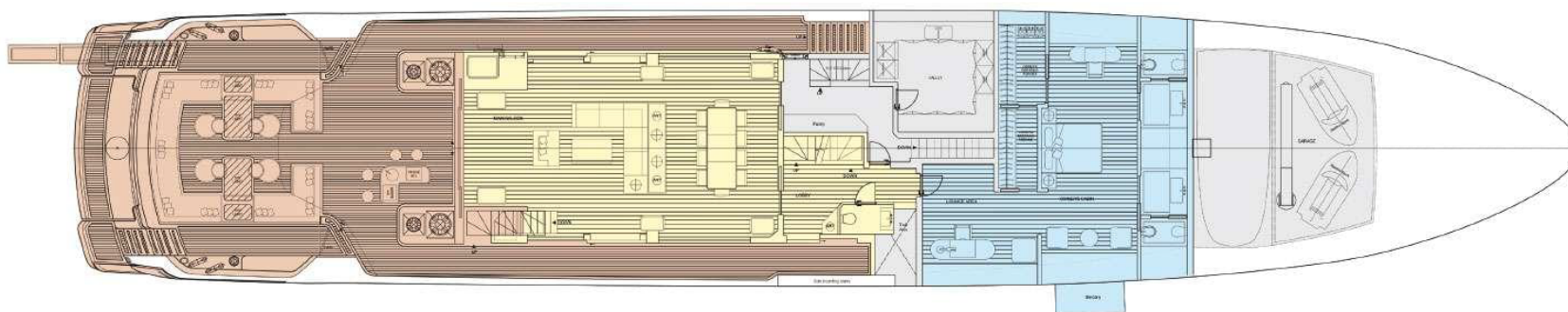
MAIN DECK
