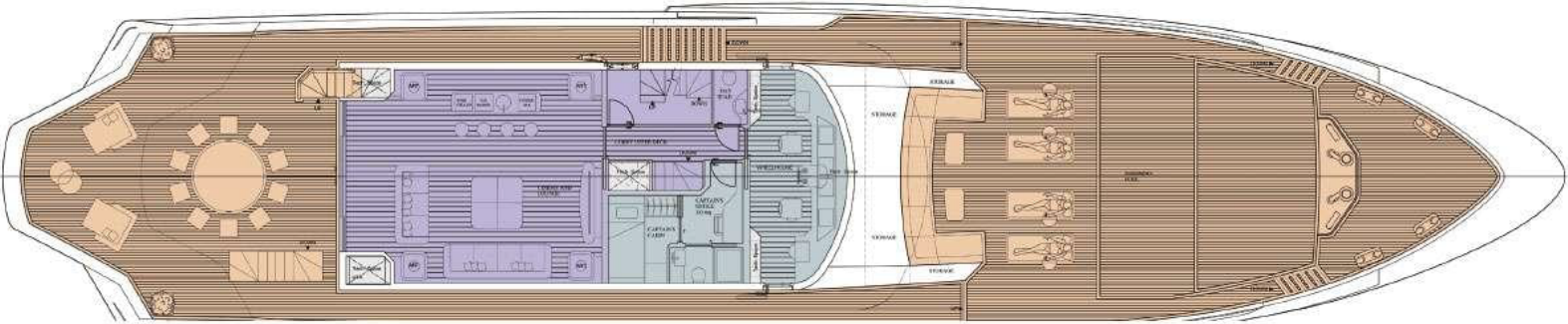
UPPER DECK
