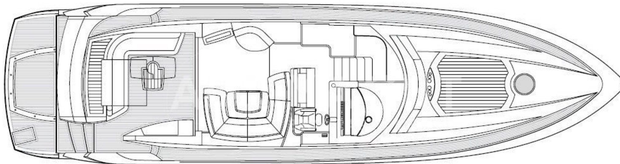
MAIN DECK
