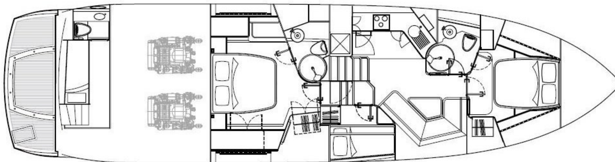
LOWER DECK
