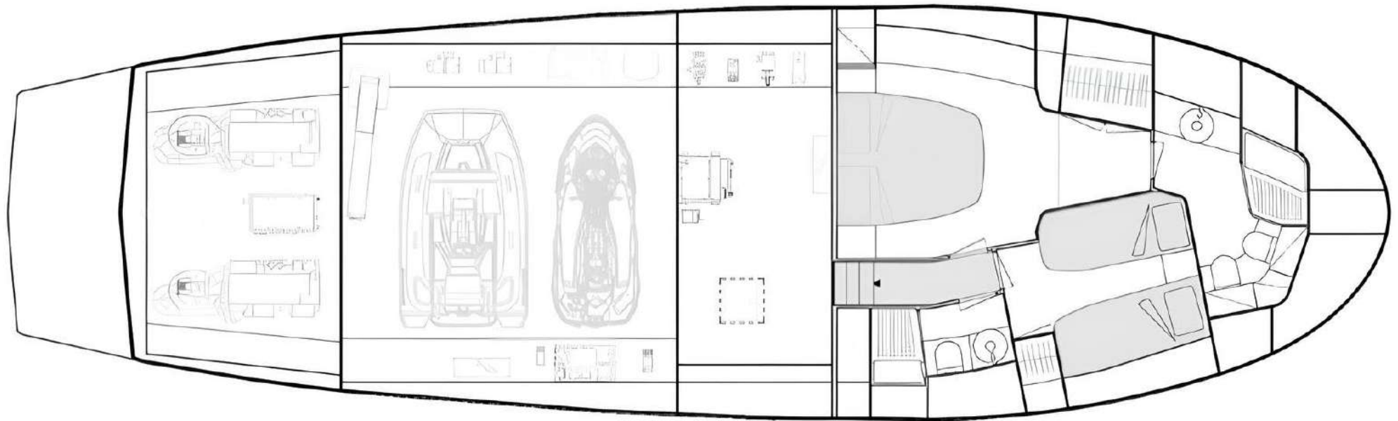
LOWER DECK
