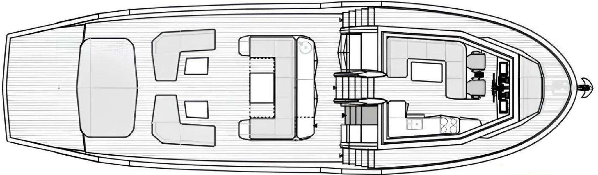
MAIN DECK
