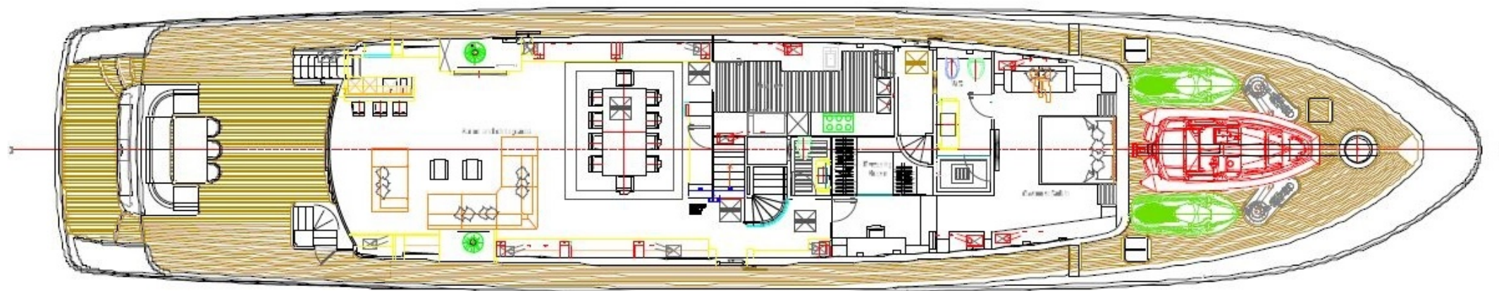
MAIN DECK
