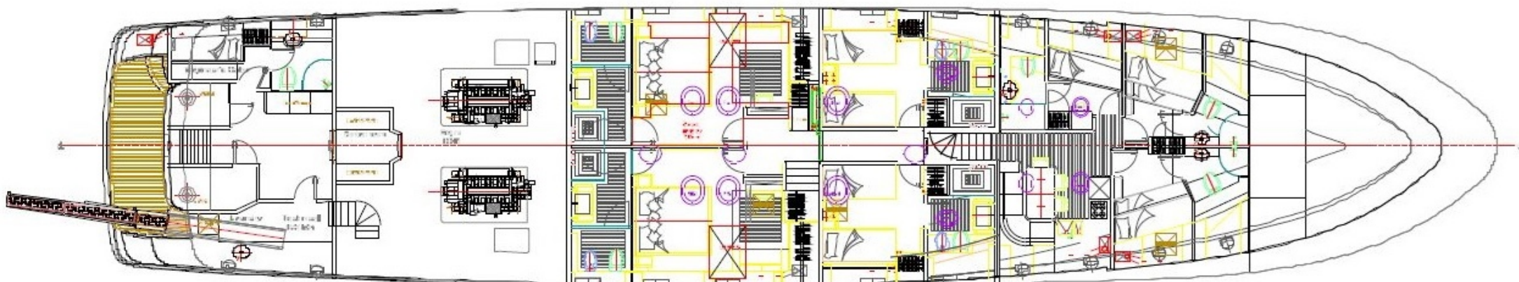
LOWER DECK
