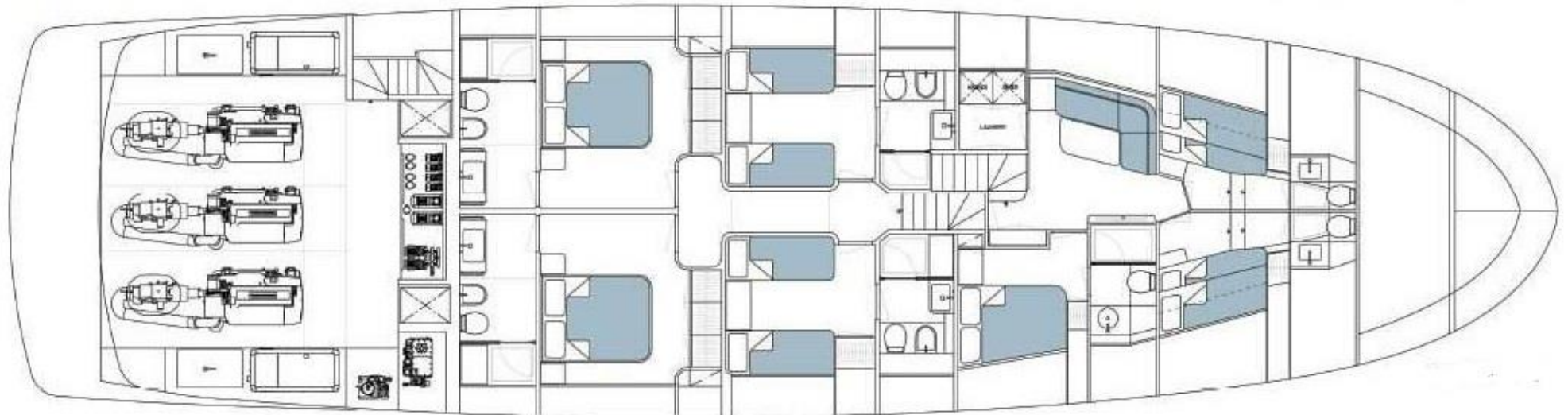
LOWER DECK
