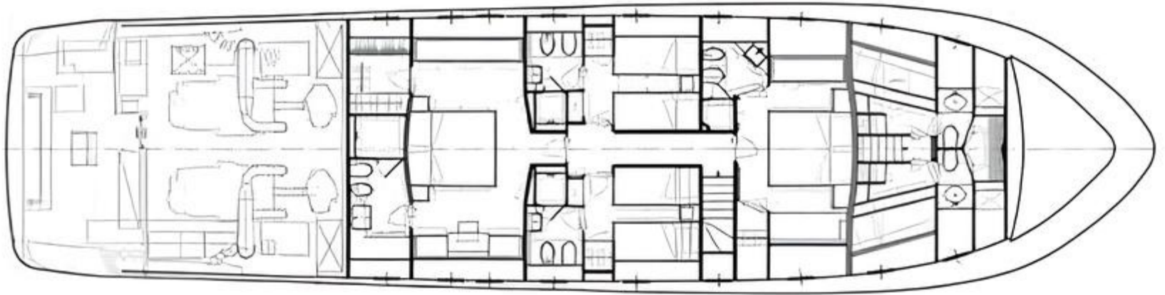
LOWER DECK
