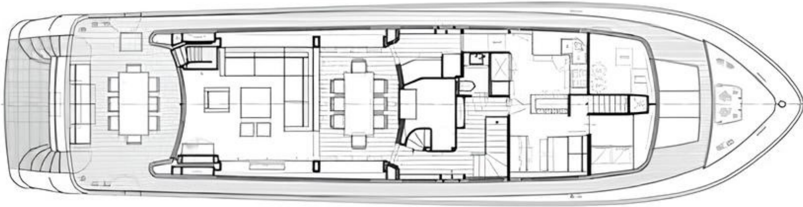
MAIN DECK
