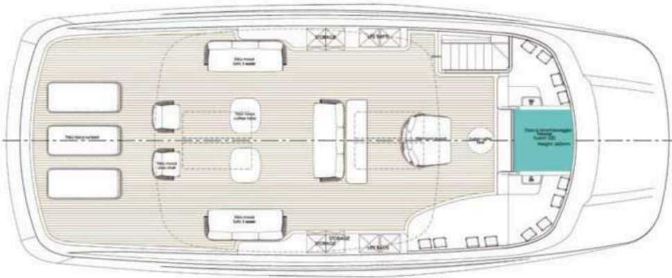
SUNDECK
